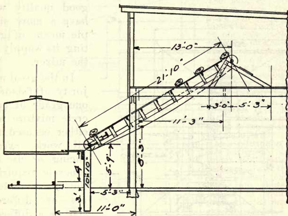
FIG. 18—SUGGESTION FOR ELEVATOR FOR CEMENT IN SACKS
